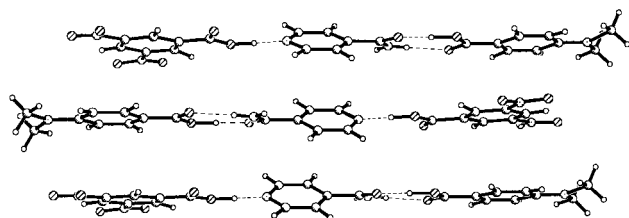
Figure 3. Side-on view of a stack of supermolecules arranged in an antiparallel fashion in 3 to illustrate the \pi(\text{weak acid})-\pi^*(\text{strong acid}) charge-transfer interactions.
